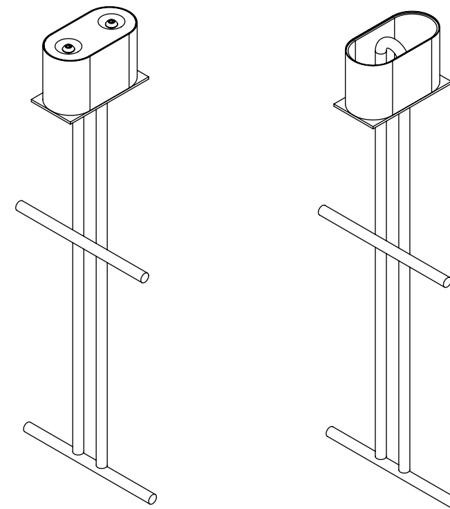
Optional Cover
